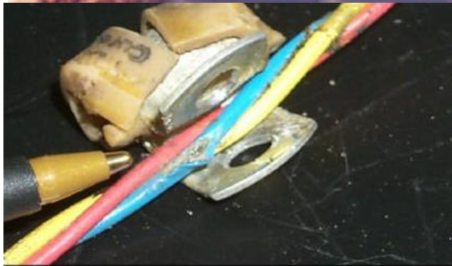
Exposed conductor under clamp, discovered during the FAA ATSRAC intrusive inspections.
