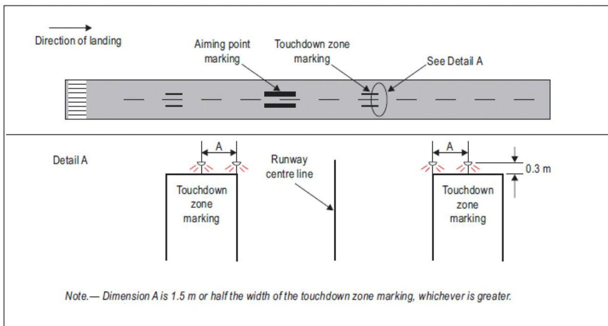
Figure M-8(C). Simple touchdown zone lighting
