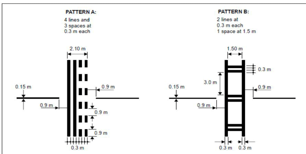
Figure L-7. Runway-holding position markings
