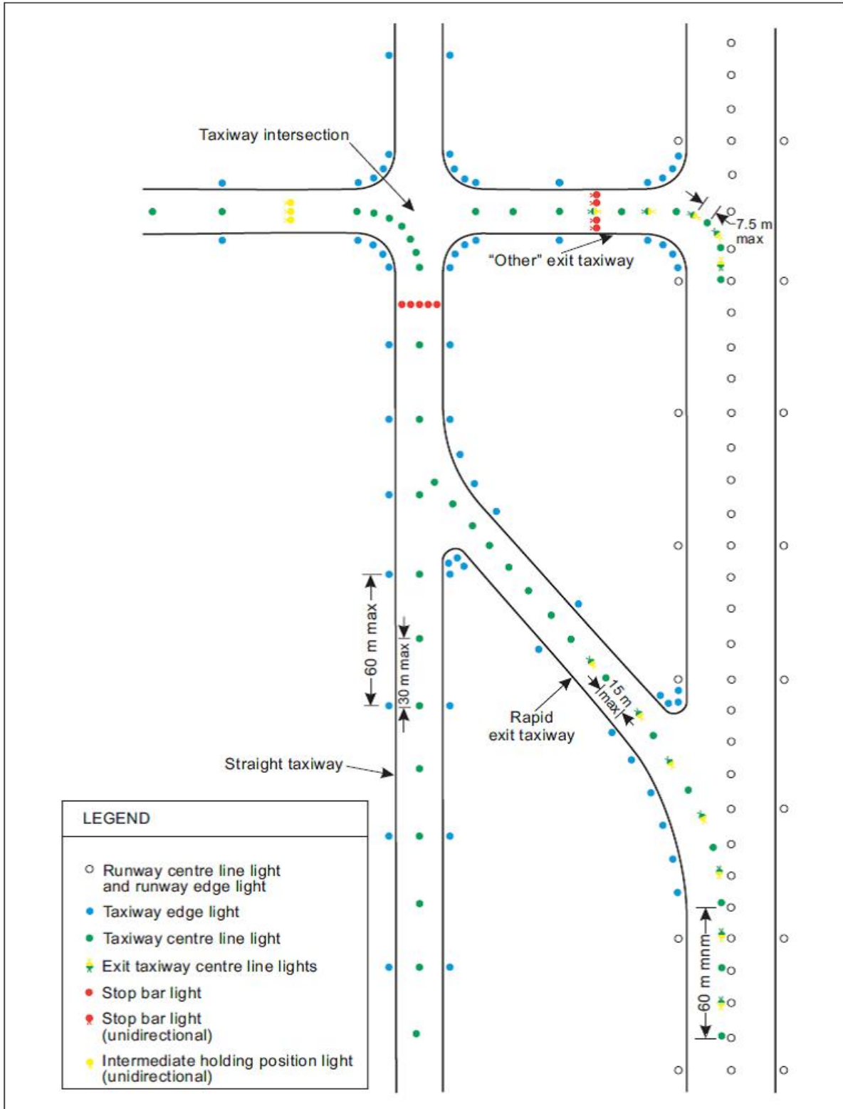
Figure M-10. Taxiway lighting
