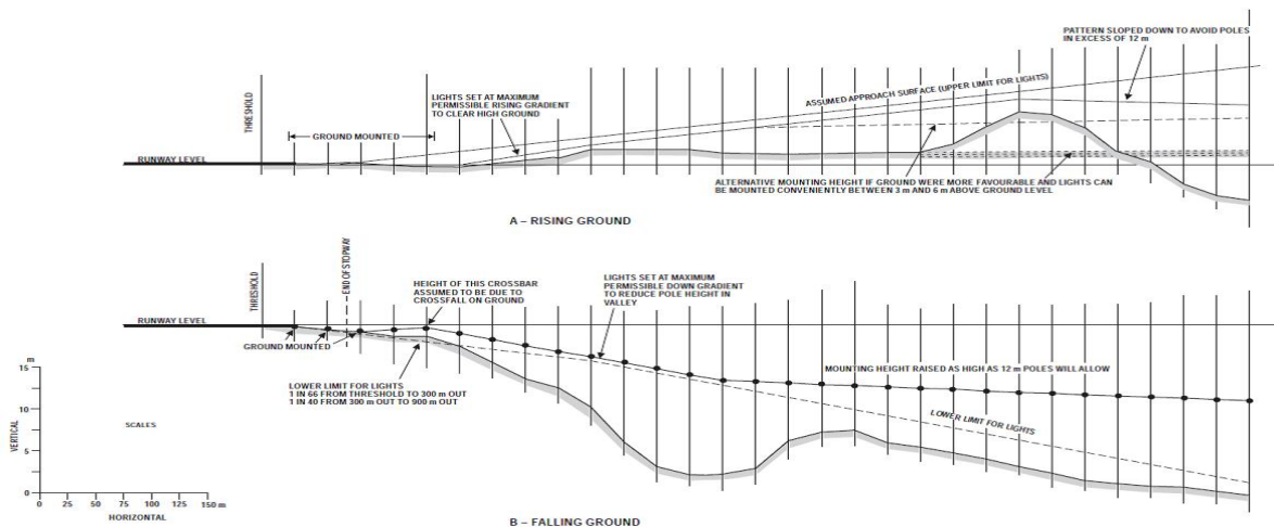
Figure GM-M-1. Vertical installation tolerances
