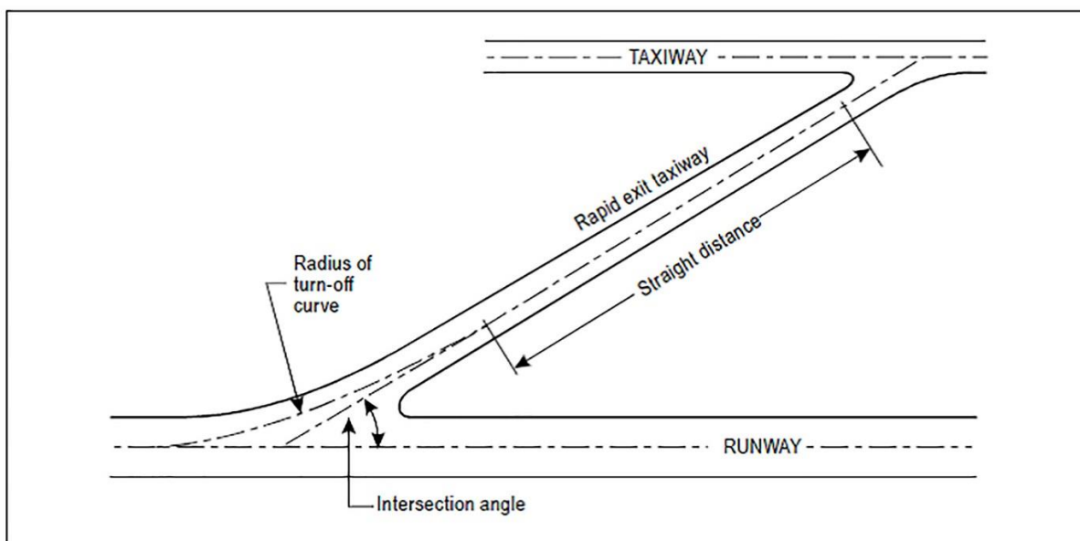
Figure D-1. Rapid exit taxiway
