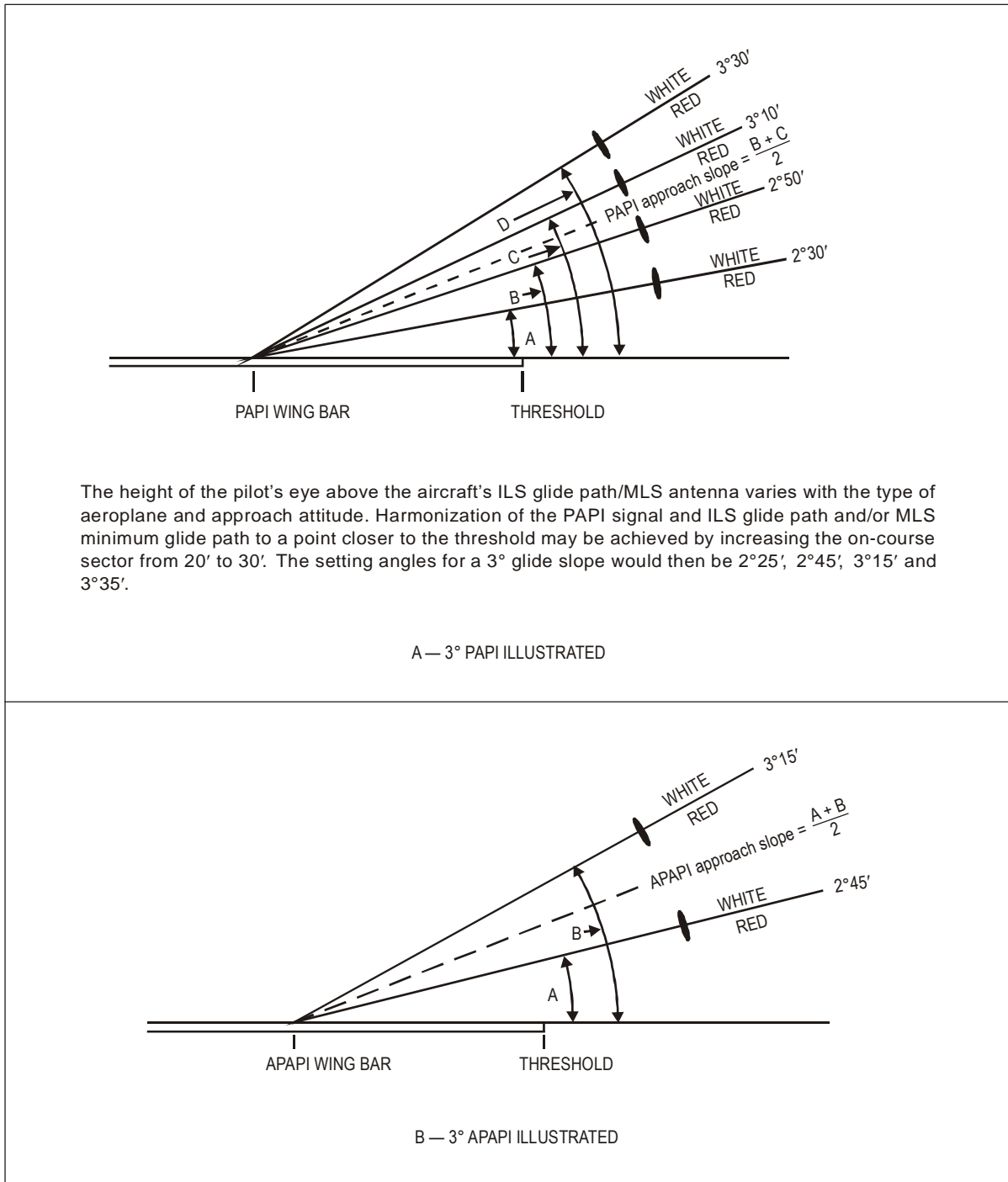
Figure M-5. Light beams and angle of elevation setting of PAPI and APAPI
