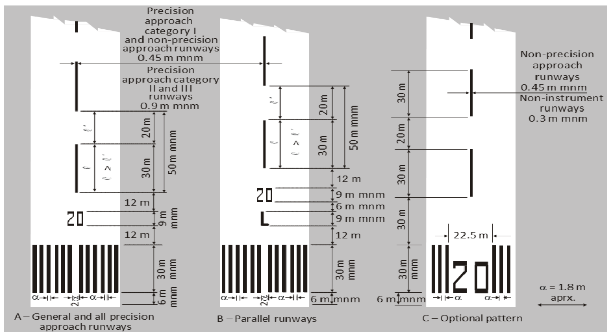
Figure L-1. Runway designation, centre line and threshold markings
