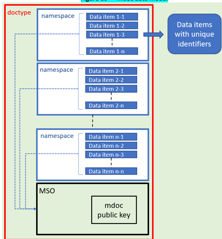
Figure 10 — Mdoc data model
