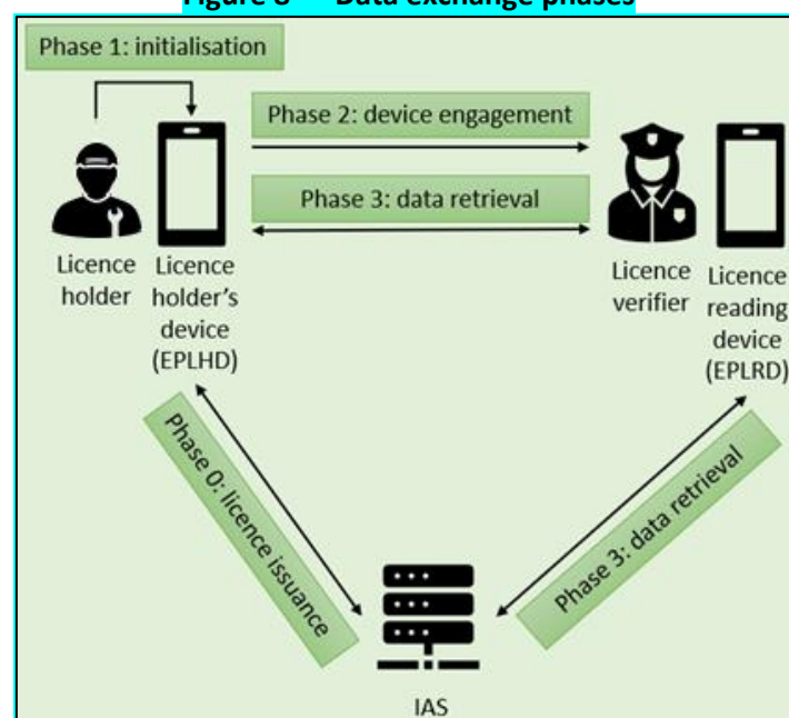
Figure 8 — Data exchange phases
