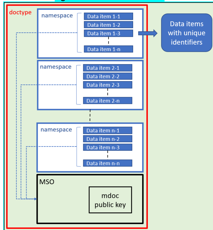
Figure 10 — Mdoc data model
