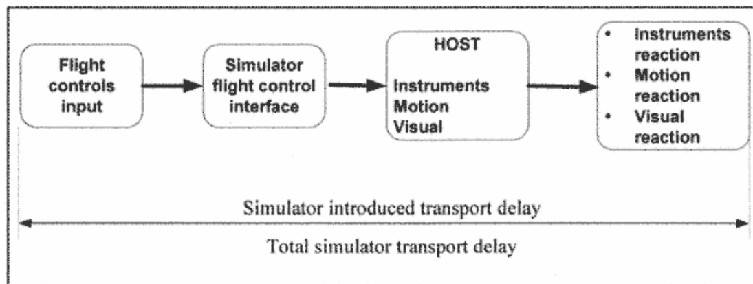
Figure A2C Transport Delay for simulation of classic non-computer controlled aircraft.
